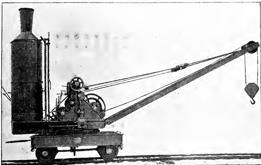
Fig. 211. LOCOMOTIVE CRANE. YALE & TOWNE MANUFACTURING COMPANY. Radius of Boom, 26 ft. 6 ins. Capacity, 10 tons. Weight 56,000 lbs. (Details are shown in Figs. 389-391.)
